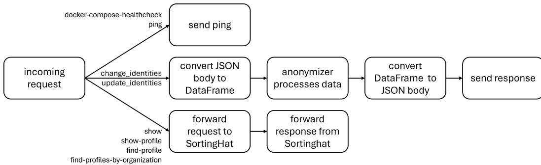
Figure 6.1: Server Diagram
