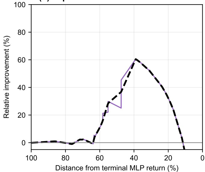
(b) Improvement vs. terminal distance
