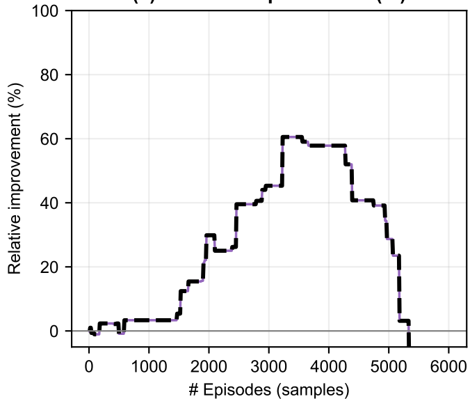
(a) Relative improvement (%)
