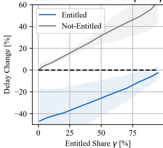
Scenario 1: In-Flow 100 [veh/h]
