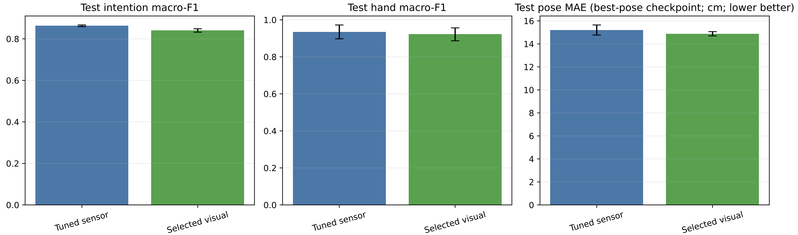
Final frozen visual comparison (mean \pm population SD; seeds 42/43/44)
