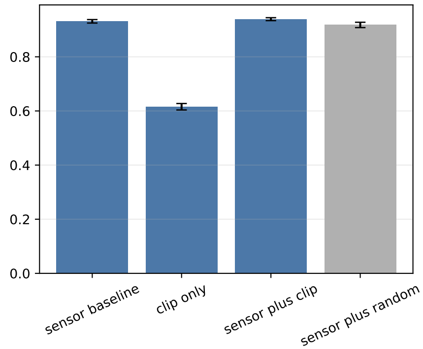
Validation intention macro-F1
