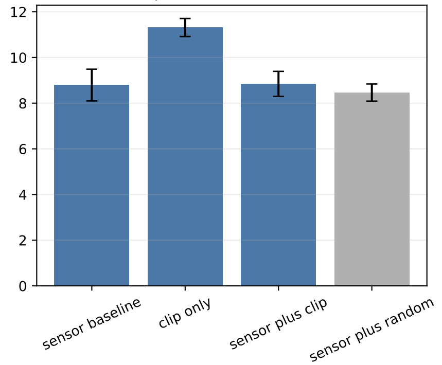
Validation pose MAE (cm) (lower better)
