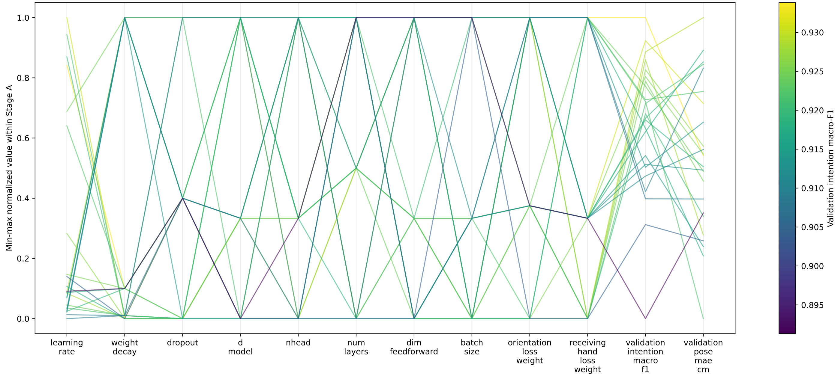
Hyperparameter search parallel coordinates
