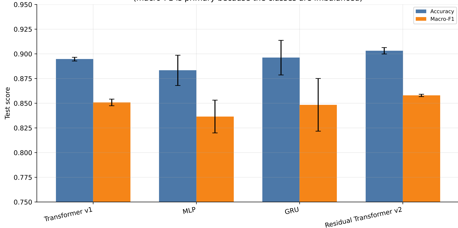
Test intention accuracy and macro-F1 (macro-F1 is primary because the classes are imbalanced)
