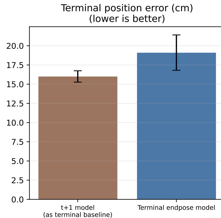
Existing t+1 predictor versus terminal-endpose training common robust terminal targets; mean \pm population SD, seeds 42/43/44
