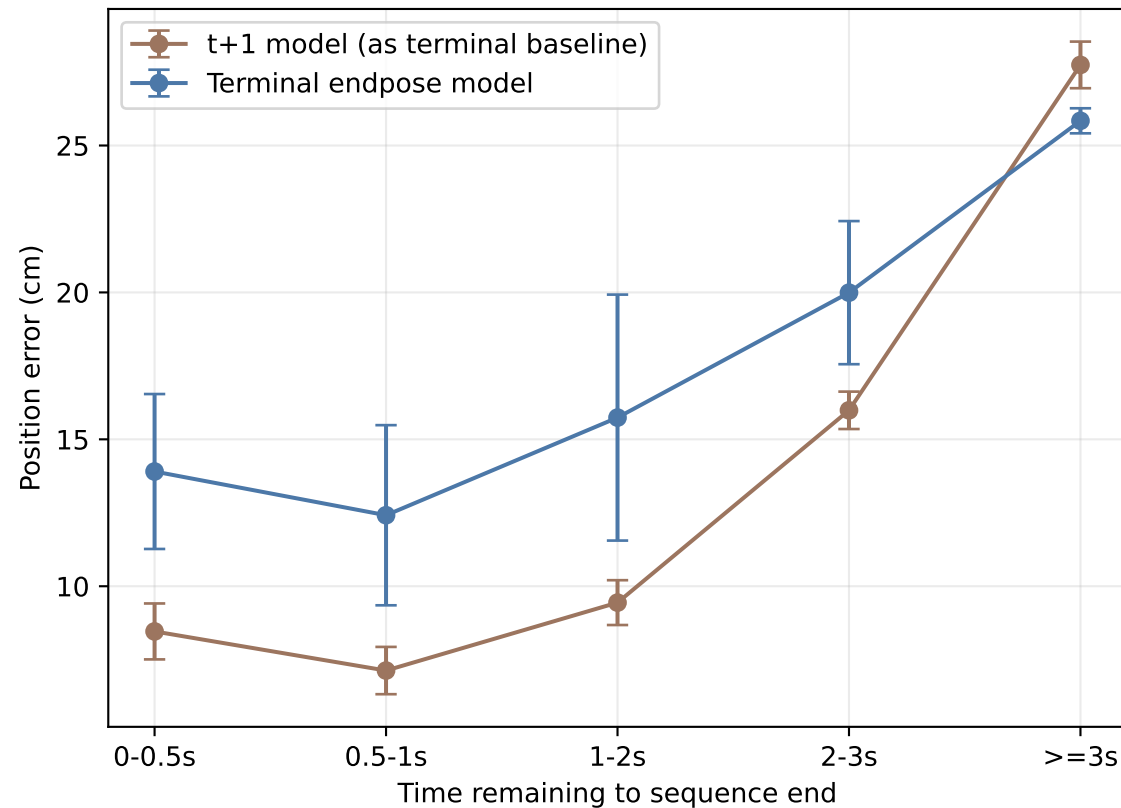
Terminal-pose error versus remaining time (oracle receiving hand)
