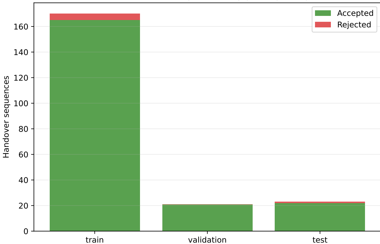
Robust terminal-target audit by participant split
