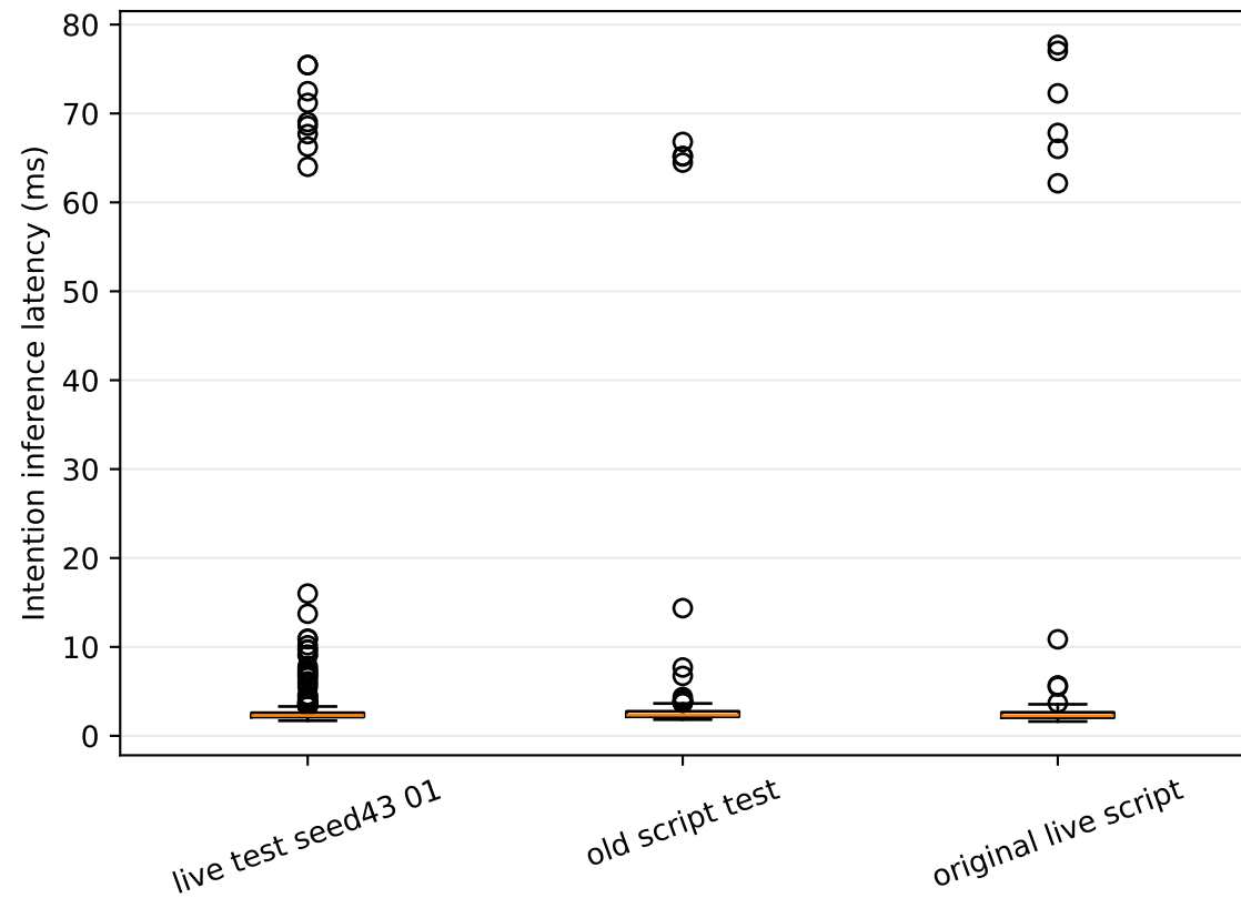
Existing Mac live sessions (exploratory; not final tuned-model benchmark)
