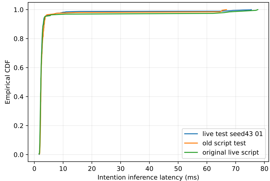
Existing Mac live sessions (exploratory; not final tuned-model benchmark)
