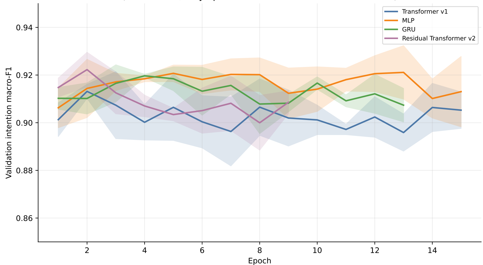
Validation intention macro-F1, mean \pm standard deviation (three seeds; only epochs available for all seeds of a model)
