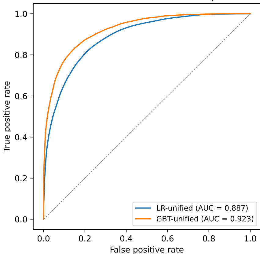
ROC: unified LR vs GBT (test split)
