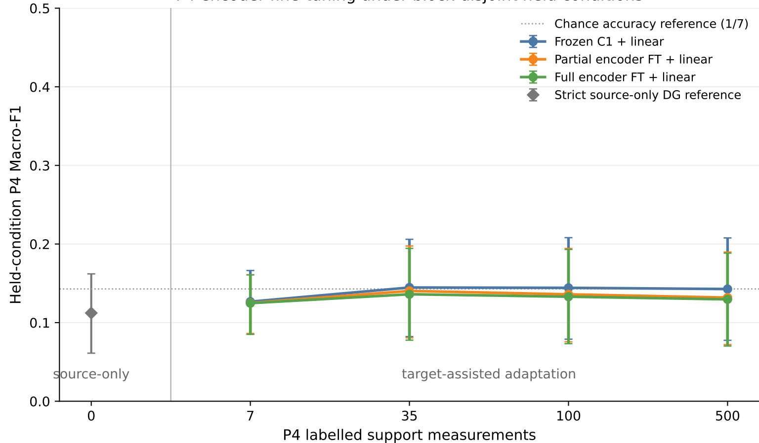
P4 encoder fine-tuning under block-disjoint held conditions
