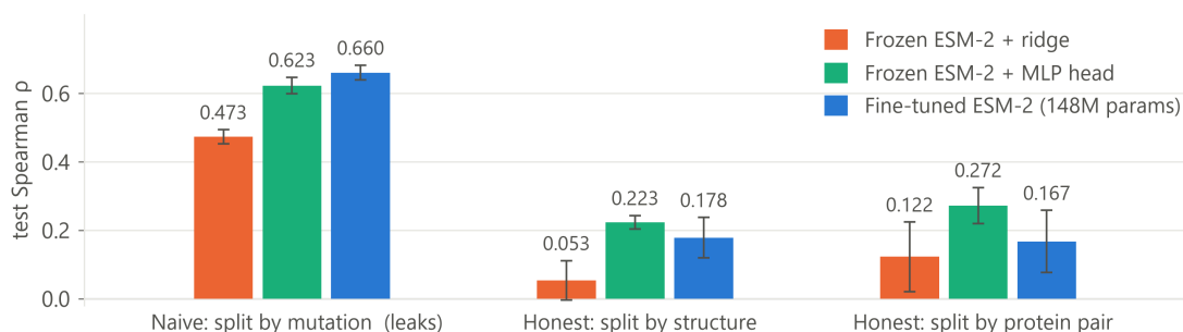
Figure 2 — the leakage gradient. Test Spearman by method under each split definition; bars are the mean of 5 replicates, whiskers \pm 1 sd. Note the within-group order too: on the leaky split more trainable parameters help monotonically; on both honest splits that ordering disappears. LoRA is absent from this figure by design — it was run on split_pdb_id only, so it has no bars to place in the other two groups.
