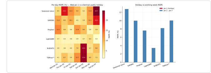
Per-day MAPE heatmap
