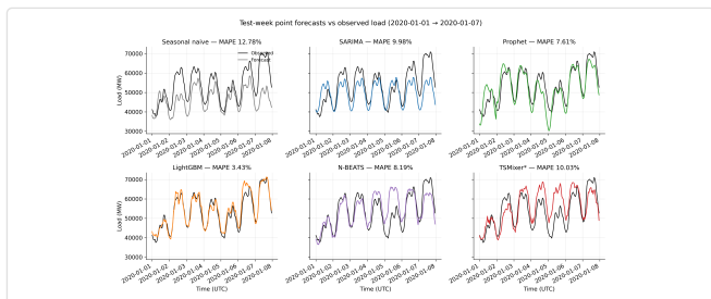
Six-model comparison
