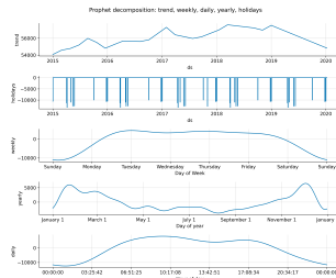
Prophet trend / seasonal decomposition
