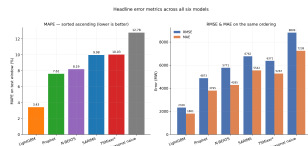
Scoreboard — MAPE, RMSE, MAE
