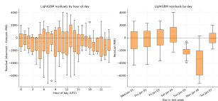
Winner residuals by hour and day
