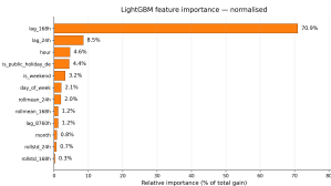
Feature importance (normalised)
