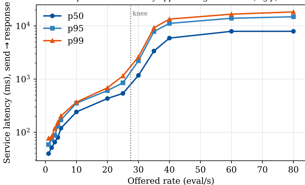
Request service latency approaching saturation (log y)
