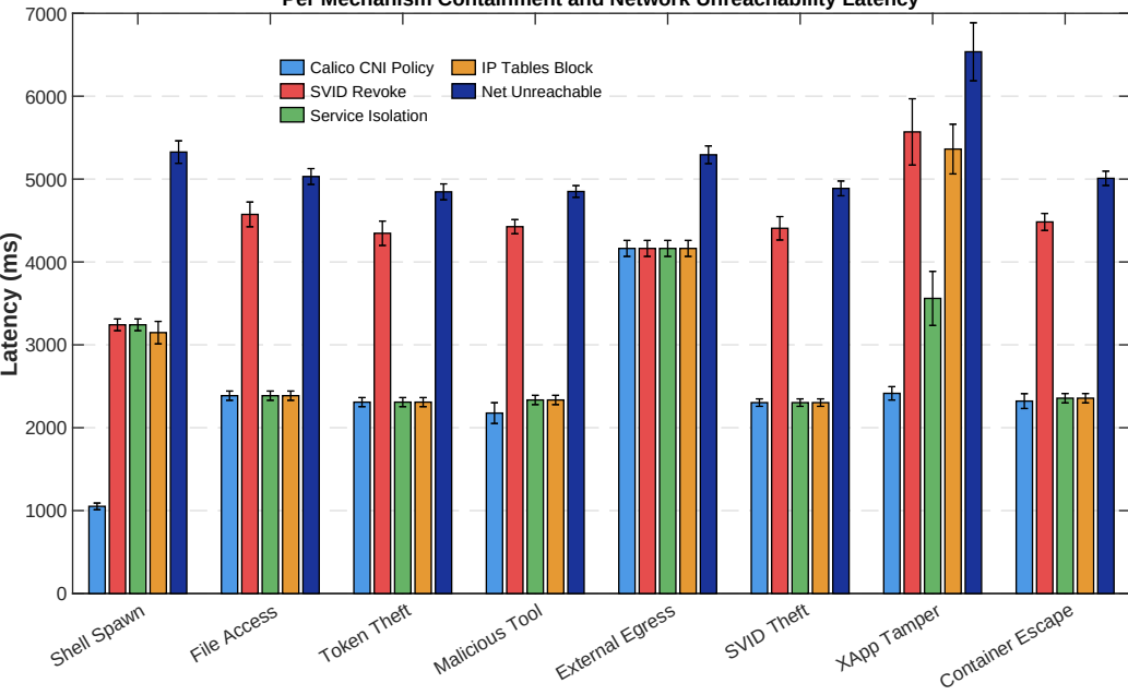
Per Mechanism Containment and Network Unreachability Latency
