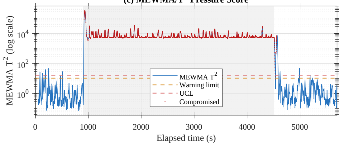
(c) MEWMA/ T^2 Pressure Score
