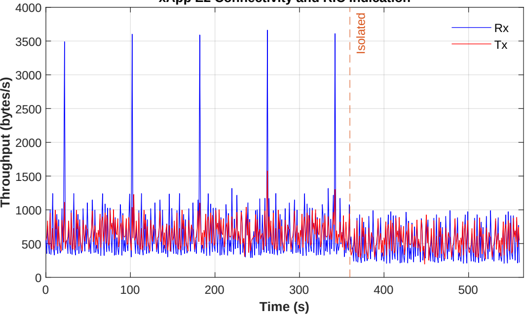
xApp E2 Connectivity and RIC Indication
