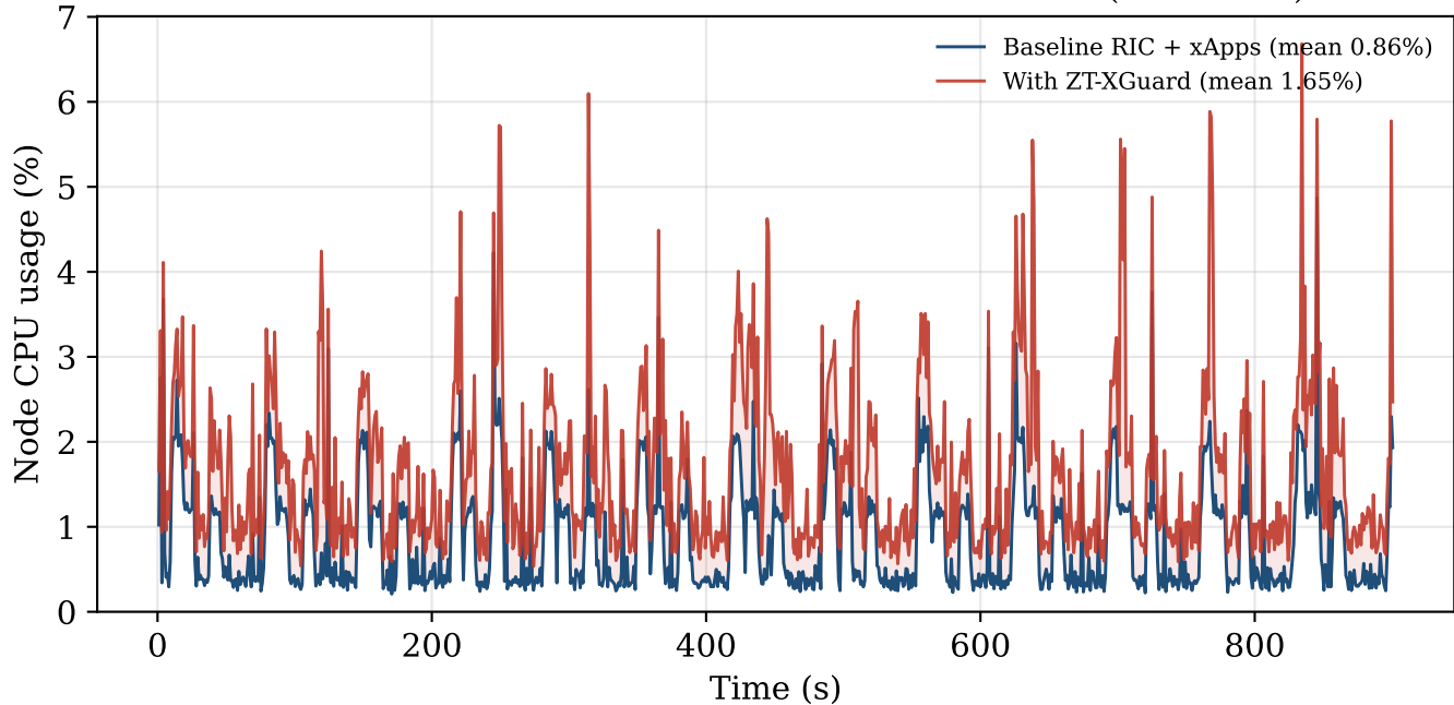
Runtime CPU overhead of ZT-XGuard on the Near-RT RIC (6-core node)
