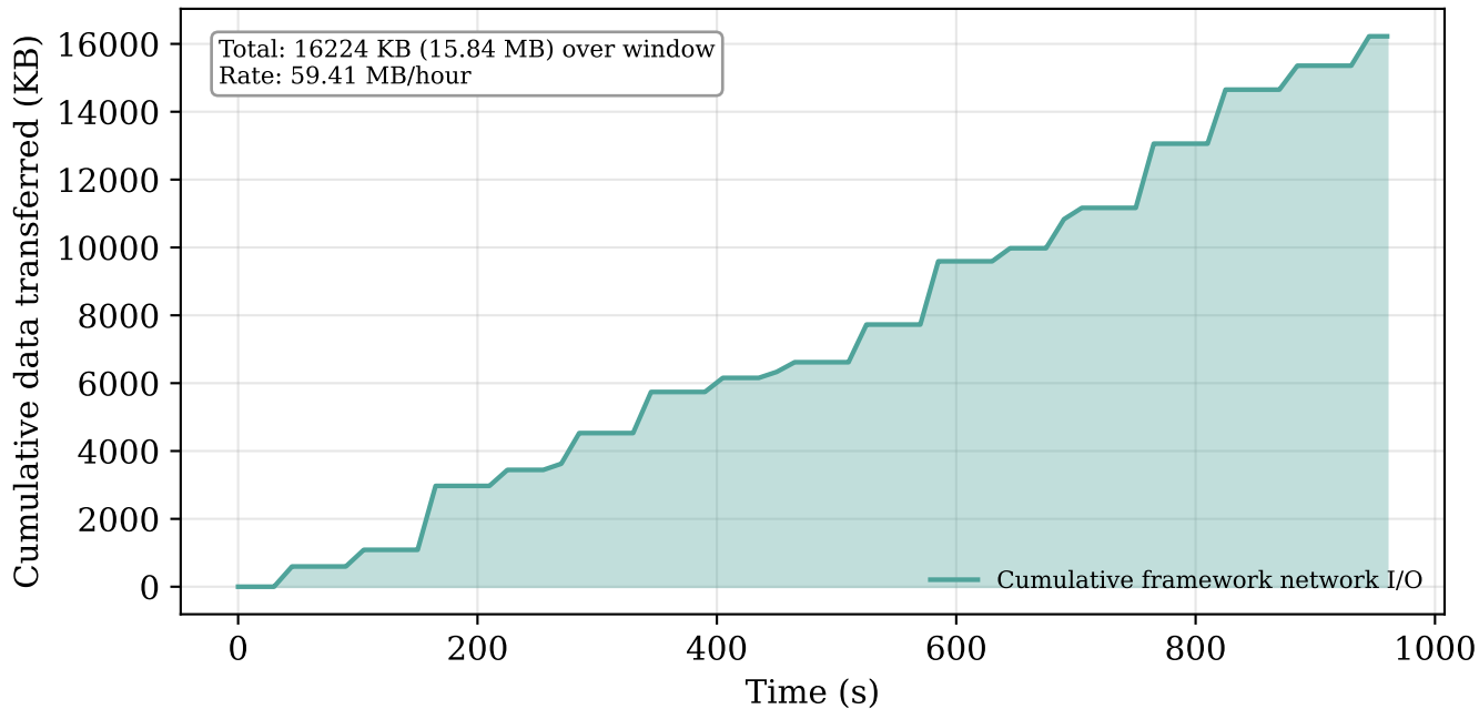
ZT-XGuard monitoring network overhead
