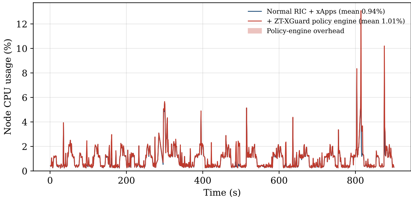
Runtime CPU overhead of the ZT-XGuard policy engine on the Near-RT RIC (6-core node)
