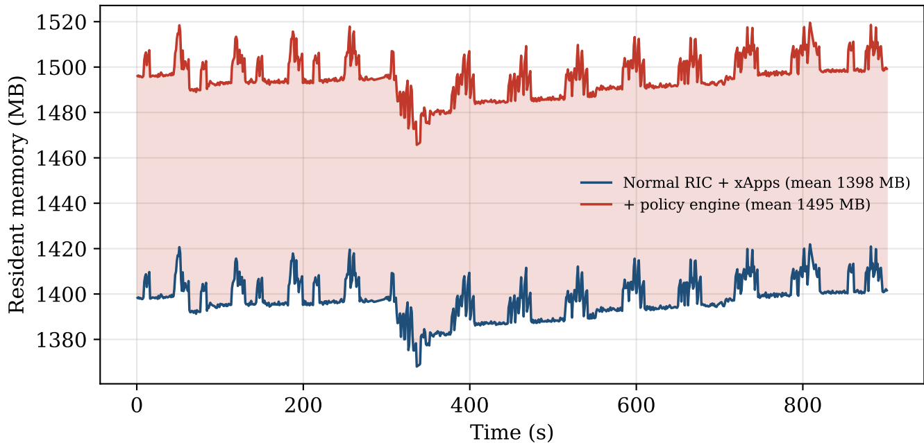
Memory: ZT-XGuard policy engine adds 98 MB
