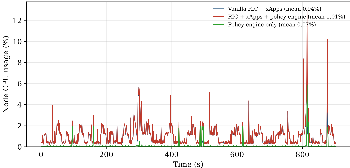
CPU usage: vanilla Near-RT RIC vs ZT-XGuard policy engine (6-core node)
