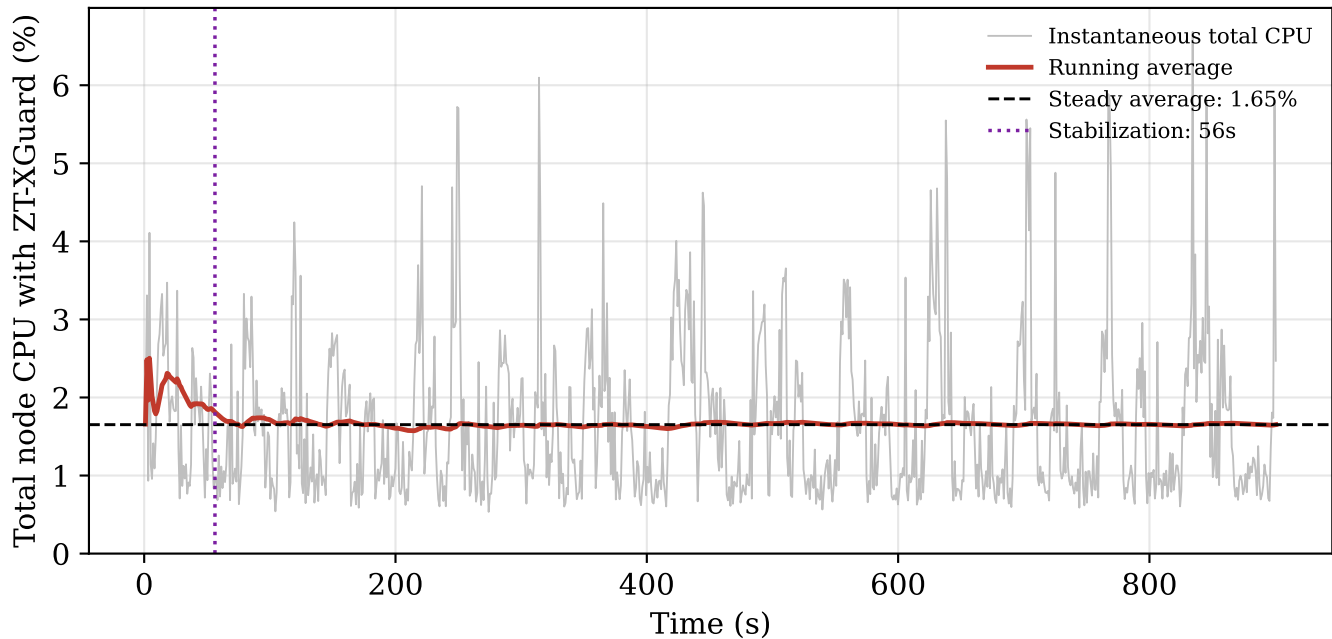
System stabilization of ZT-XGuard runtime overhead
