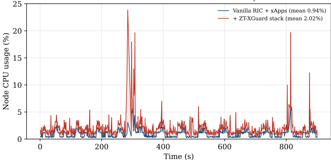
CPU: vanilla Near-RT RIC vs full ZT-XGuard security stack
