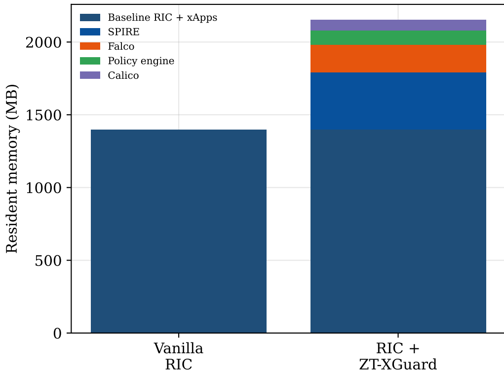
Memory: +754 MB security stack
