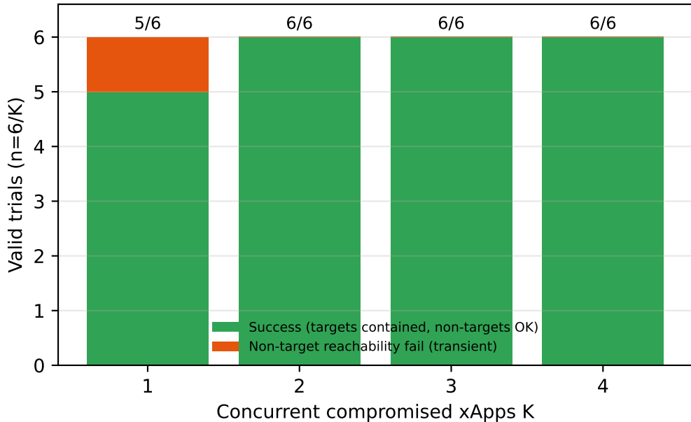
Non-target correctness by concurrency (Exp3, 24 valid trials)
