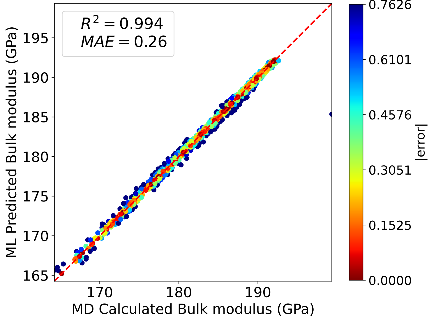
MLP (test)
