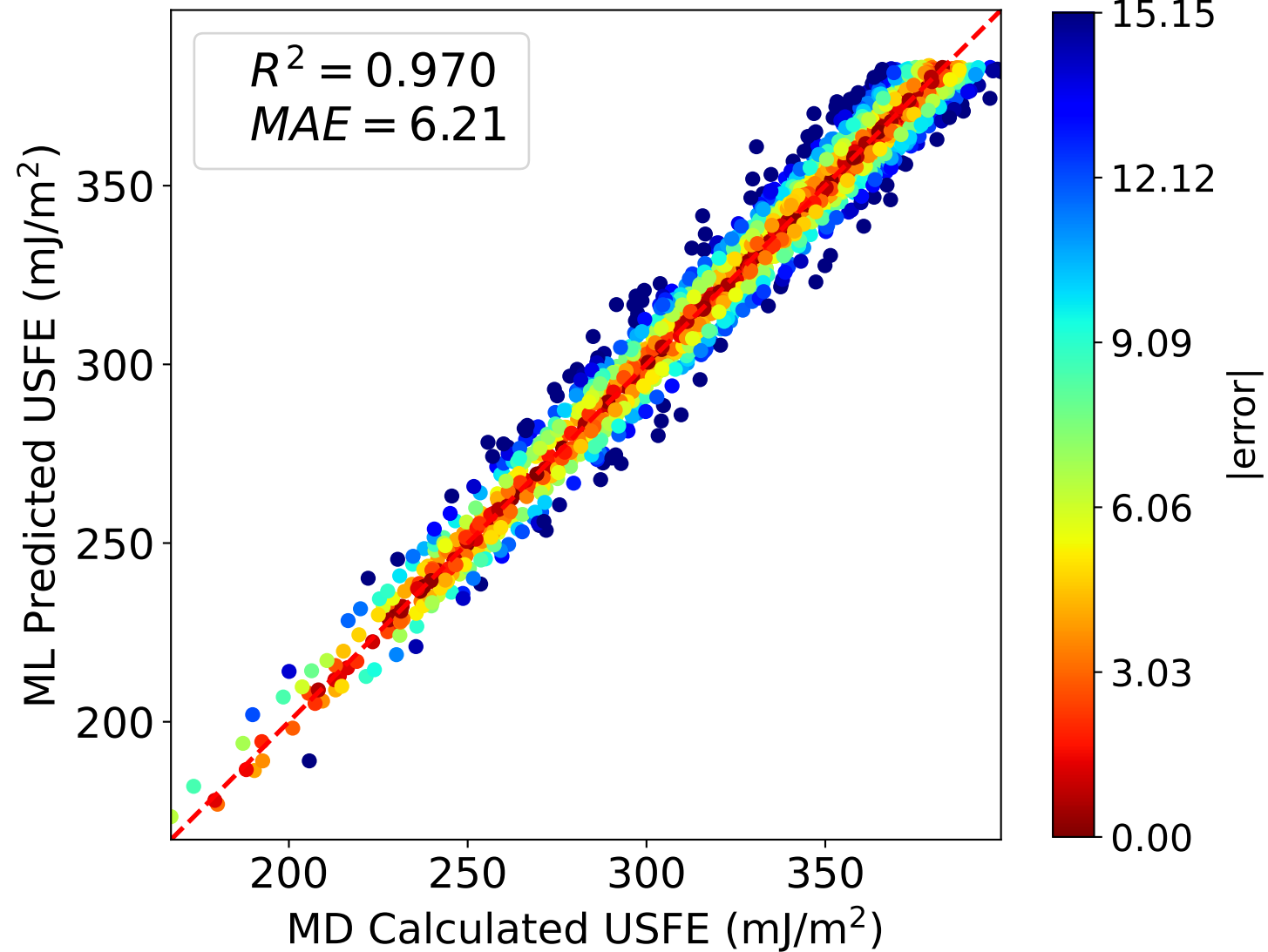
MLP (test)
