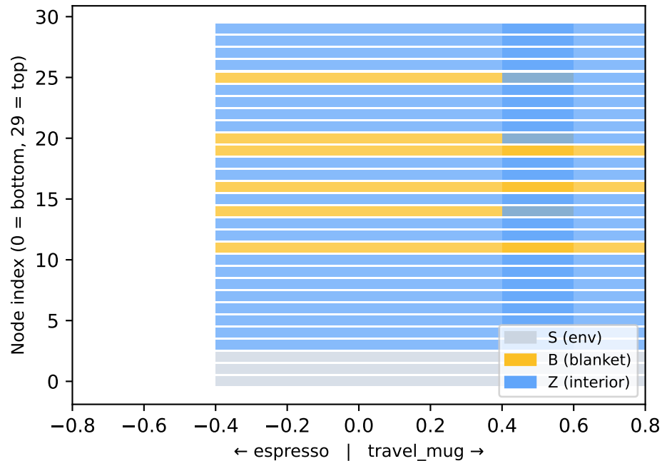
B | Inferred partitions from same flat data Different requirements \rightarrow different topology
