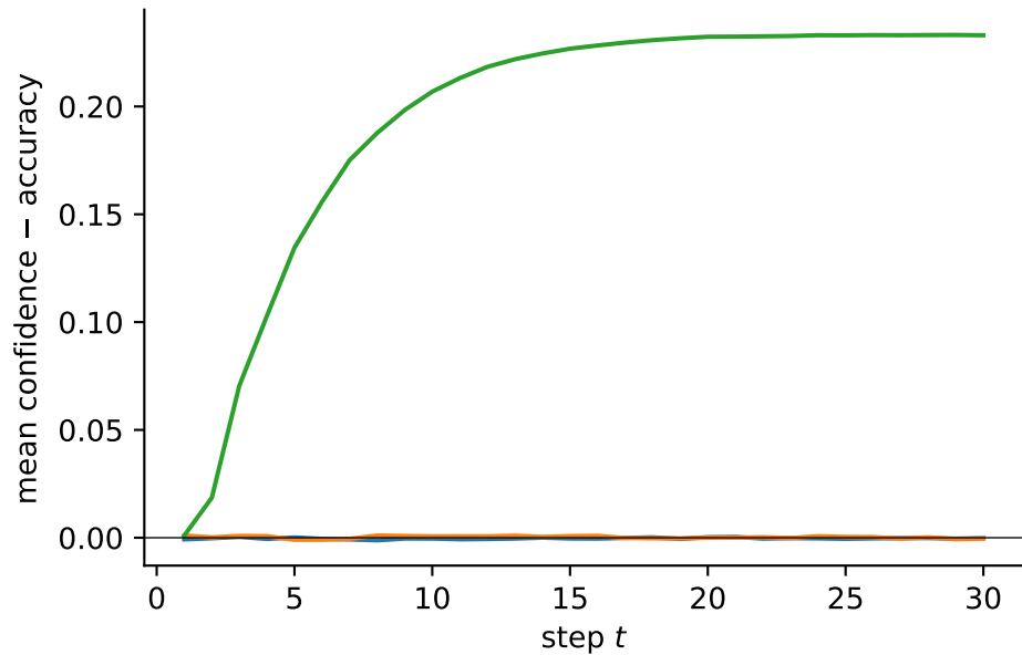
(b) Overconfidence
