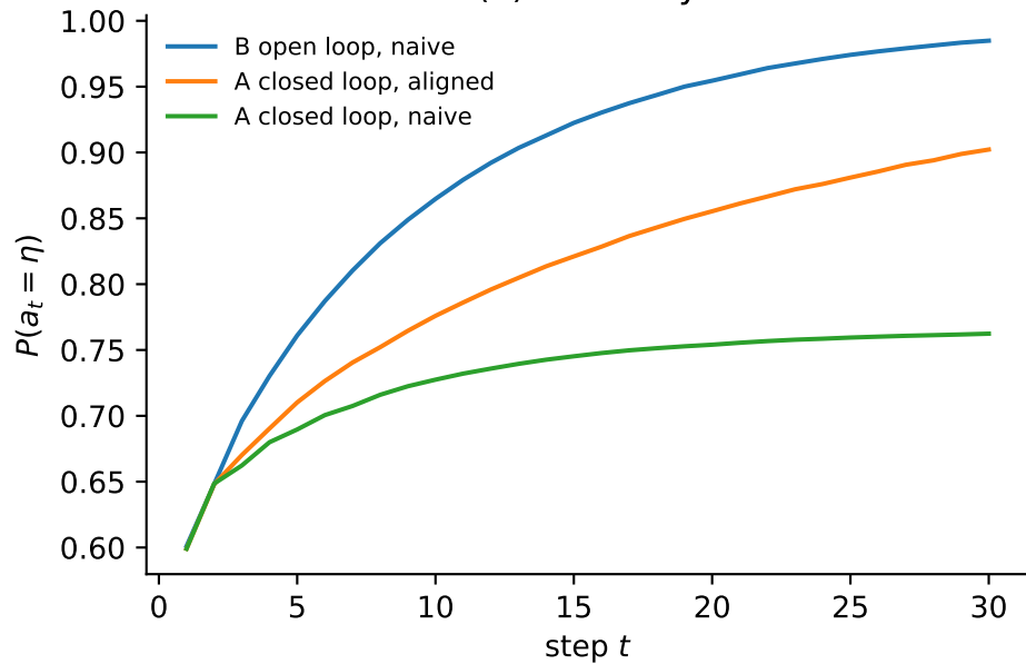
(a) Accuracy
