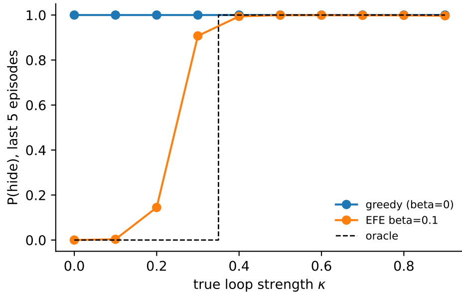
(b) Learned boundary policy
