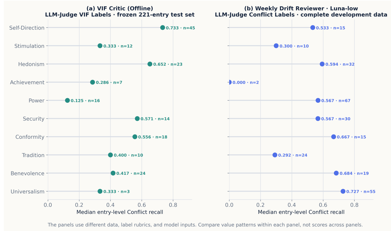
Figure 5: Per-value entry-level Conflict recall under the two completed but non-comparable evaluation regimes. The VIF Critic (Offline) panel uses LLM-Judge VIF Labels on the frozen 221-Journal-Entry test set; the Luna-low panel uses LLM-Judge Conflict Labels on complete development data. Each label gives median recall and Conflict support.
