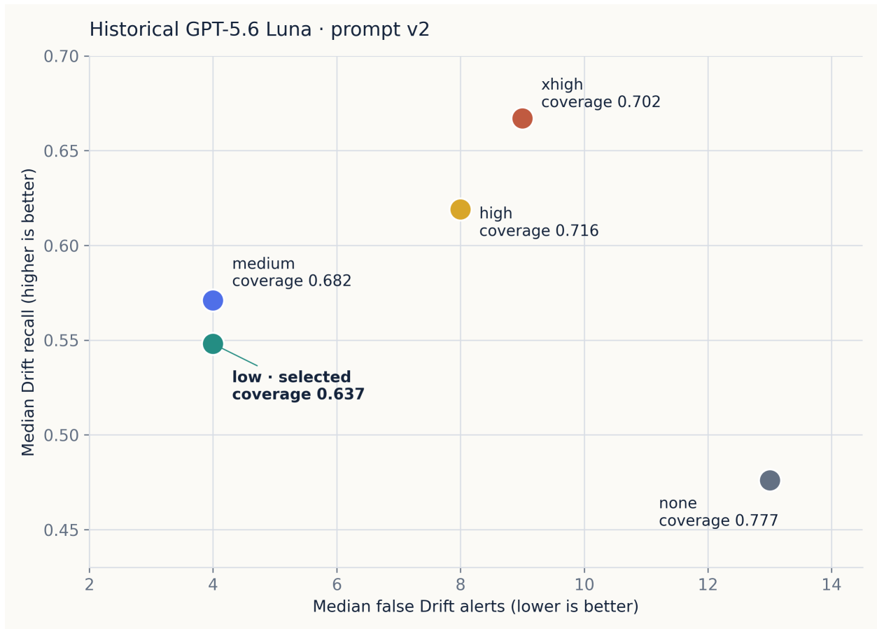
Figure 10: Historical GPT-5.6 Luna prompt-v2 operating points on AI-reviewed synthetic development data. Each marker has an exact trajectory-coverage label; marker area carries no additional quantity. Low was the selected operating point for that study.
