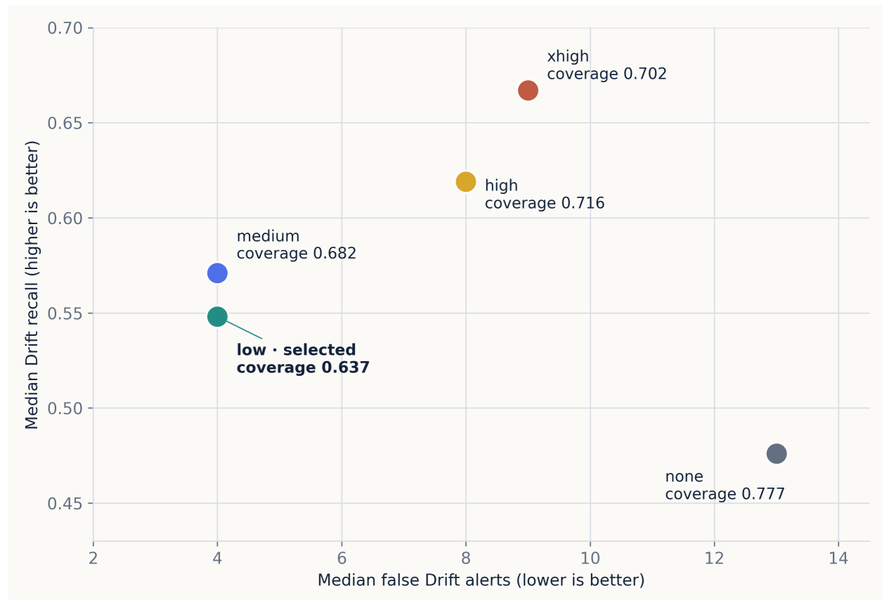
Figure 8: Weekly Drift Reviewer operating points on AI-reviewed synthetic development data. Each marker has an exact trajectory-coverage label; marker area carries no additional quantity. Twinkl retains low reasoning effort as the fixed capstone contract.
