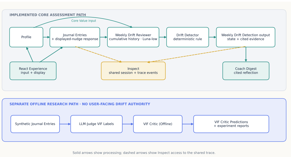
Figure 1: Adopted Twinkl architecture. The upper lane shows the implemented core assessment path and shared trace; the blue lane shows the separate offline research path. No arrow links VIF Critic Predictions to Weekly Drift Detection.
