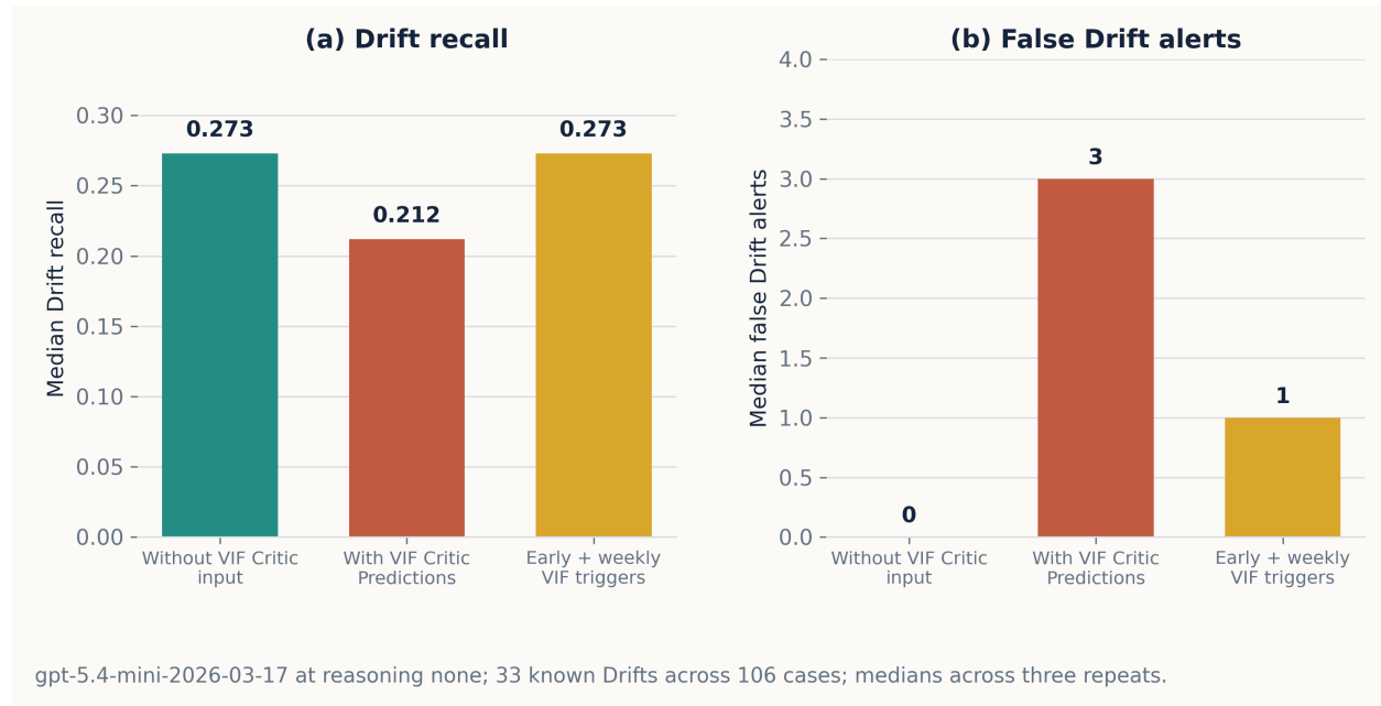
Figure 5: VIF Critic (Offline) hand-off ablation on the 33-Drift development union. All setups used gpt-5.4-mini-2026-03-17 at no reasoning effort for three repeats. Raw VIF Critic Predictions numerically lowered median Drift recall, but the paired interval included zero; early scheduling changed delay without increasing Drift hits.
