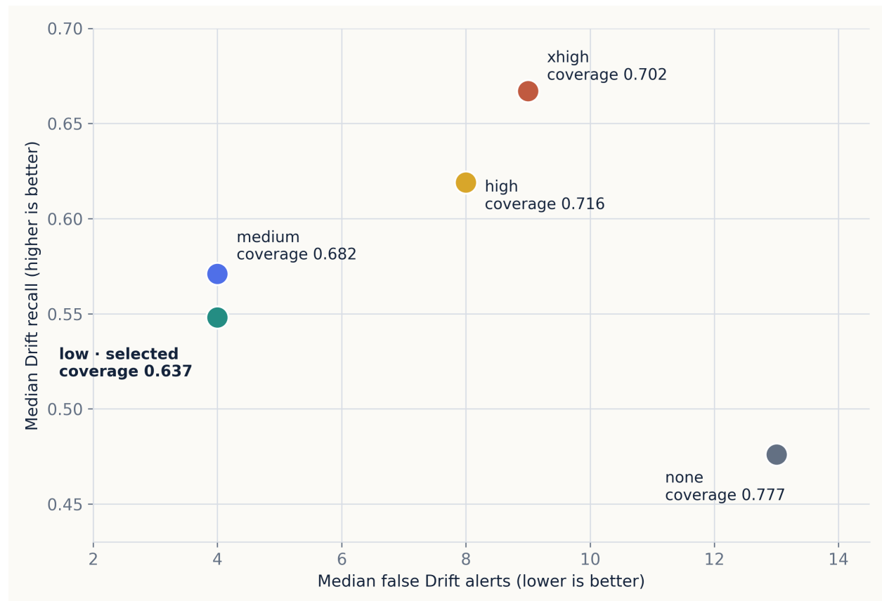
Figure 6: Weekly Drift Reviewer operating points on AI-reviewed synthetic development data. Each marker has an exact coverage label; marker area carries no additional quantity. Twinkl retains low reasoning effort as the fixed capstone contract.
