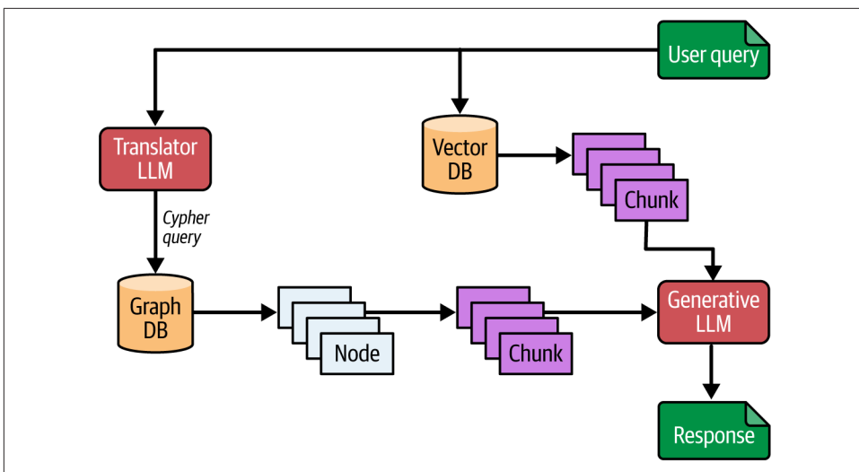
Figure 9-3. Graph query generation in a RAG pipeline
