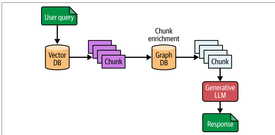
Figure 9-2. Chunk enrichment workflow: the initial chunks that are retrieved from the vector DB are then enriched using the Graph DB, before being sent over to the generative LLM step
