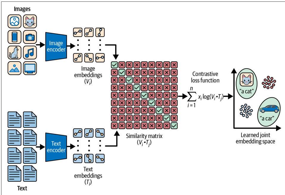
Figure 8-6. Contrastive loss training procedure
