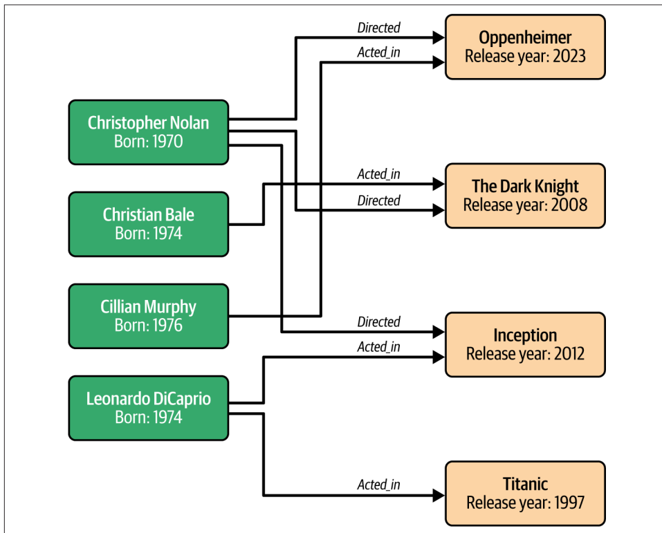
Figure 9-1. Example of a knowledge graph for movies
