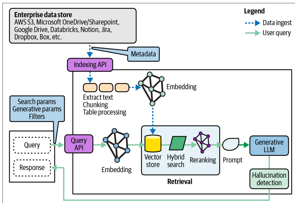
Figure 1-2. The RAG stack
