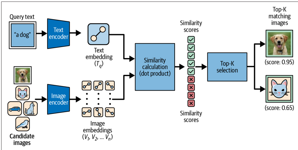
Figure 8-7. Typical inference flow in shared embeddings
