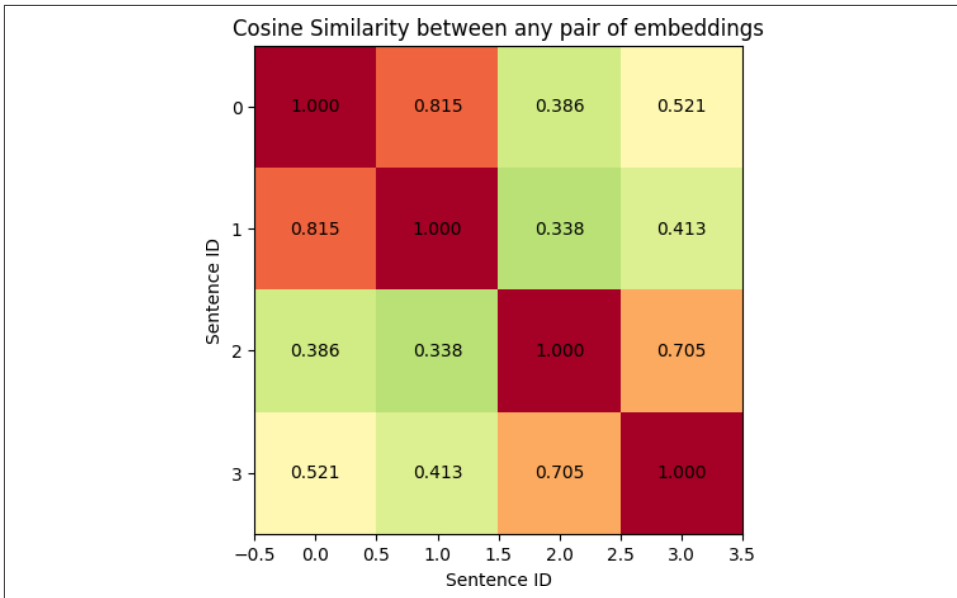
Figure 2-3. Cosine similarity between embeddings of sentences used in the coding example above
