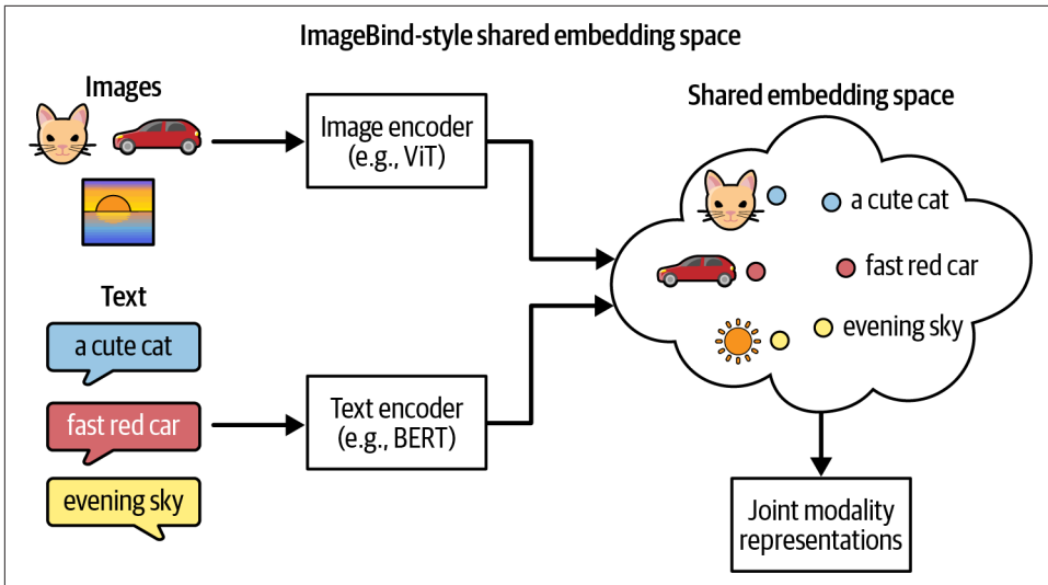
Figure 8-5. Shared embedding space for text and images
