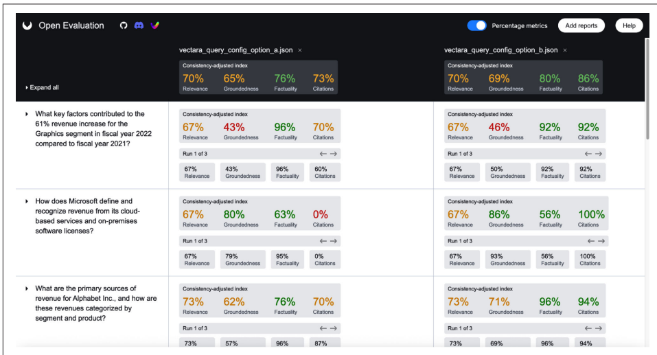
Figure 6-1. Example user interface from Open Evaluation—an app to visualize Open RAG Eval outputs, to better understand issues with RAG retrieval, generation, groundedness, or citations
