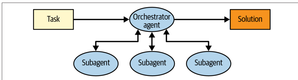
Figure 7-4. The orchestrator–worker multi-agent pattern: the orchestrator agent is responsible for the overall task completion, outsourcing pieces to specialized subagents
