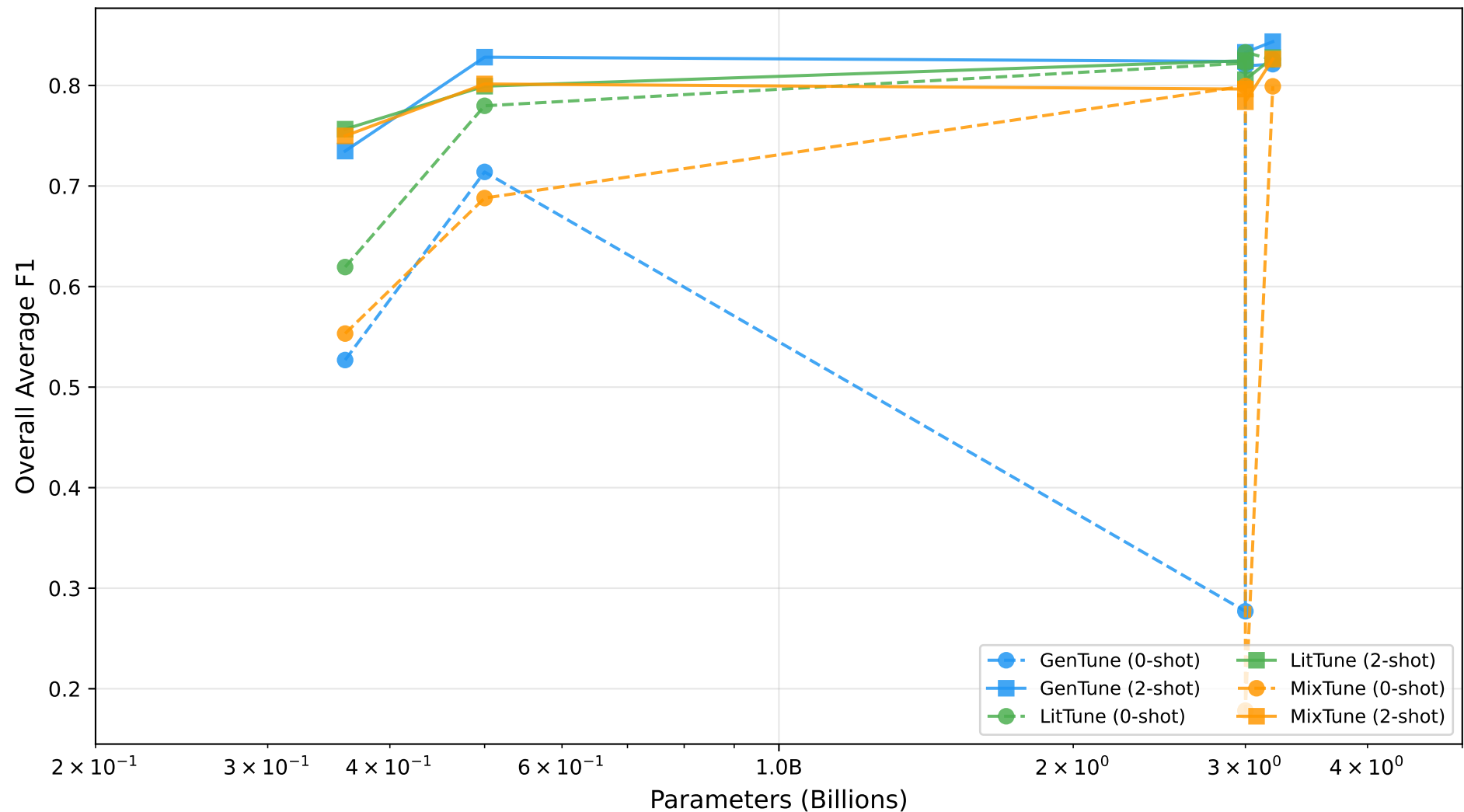
Scaling Trends: Overall Avg F1 by Model Size
