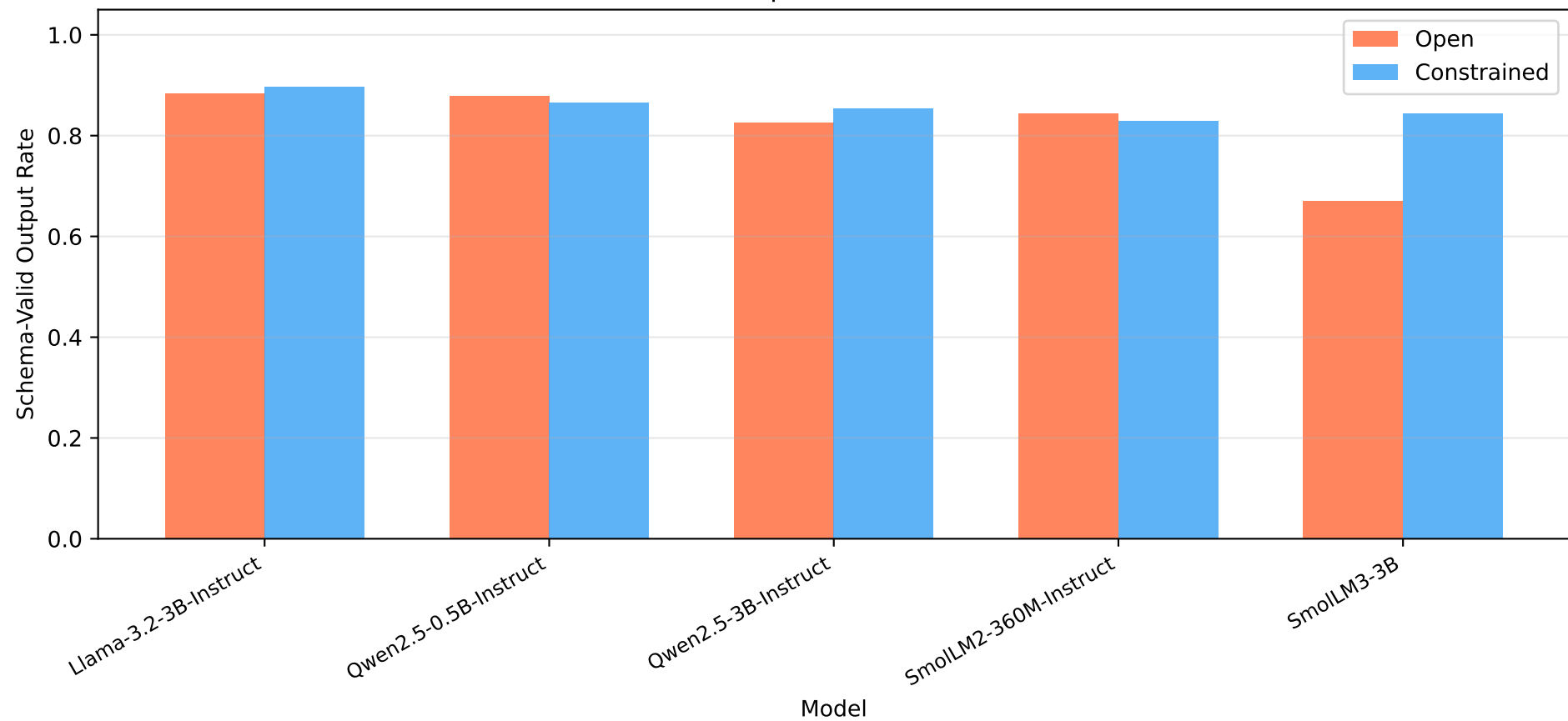
Schema-Valid Rate: Open vs Constrained Generation
