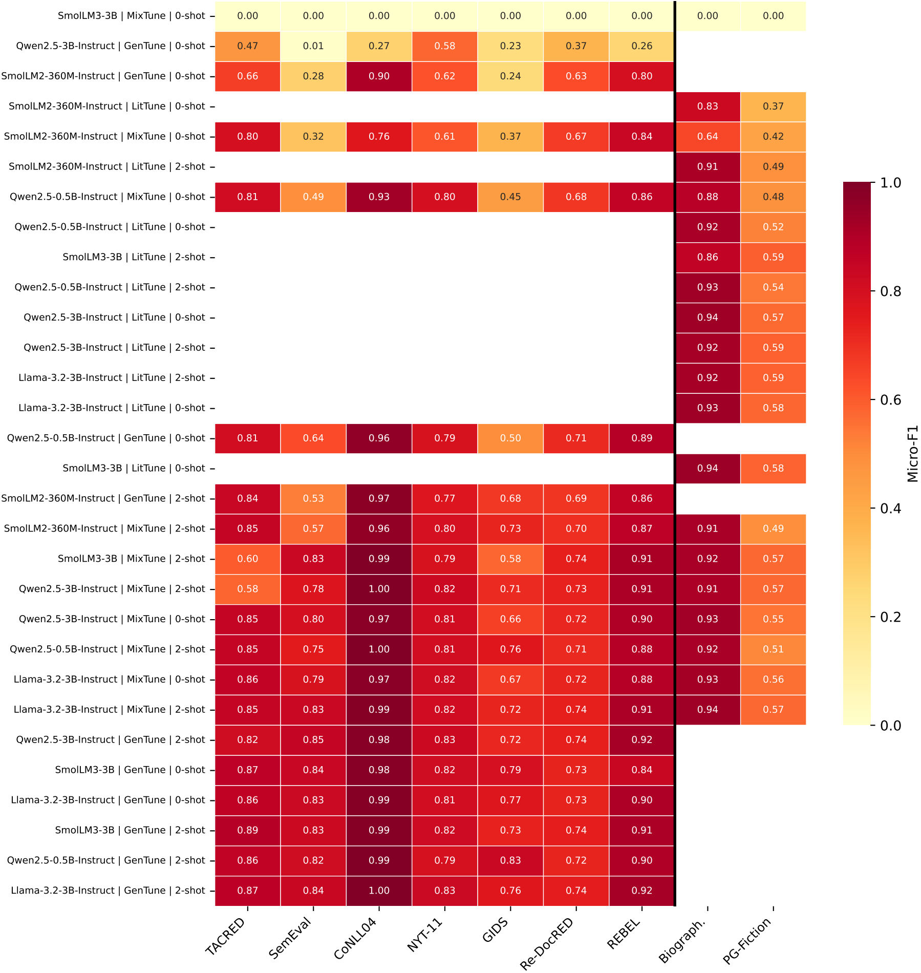
Per-Dataset Micro-F1 for All Tuned SLMs
