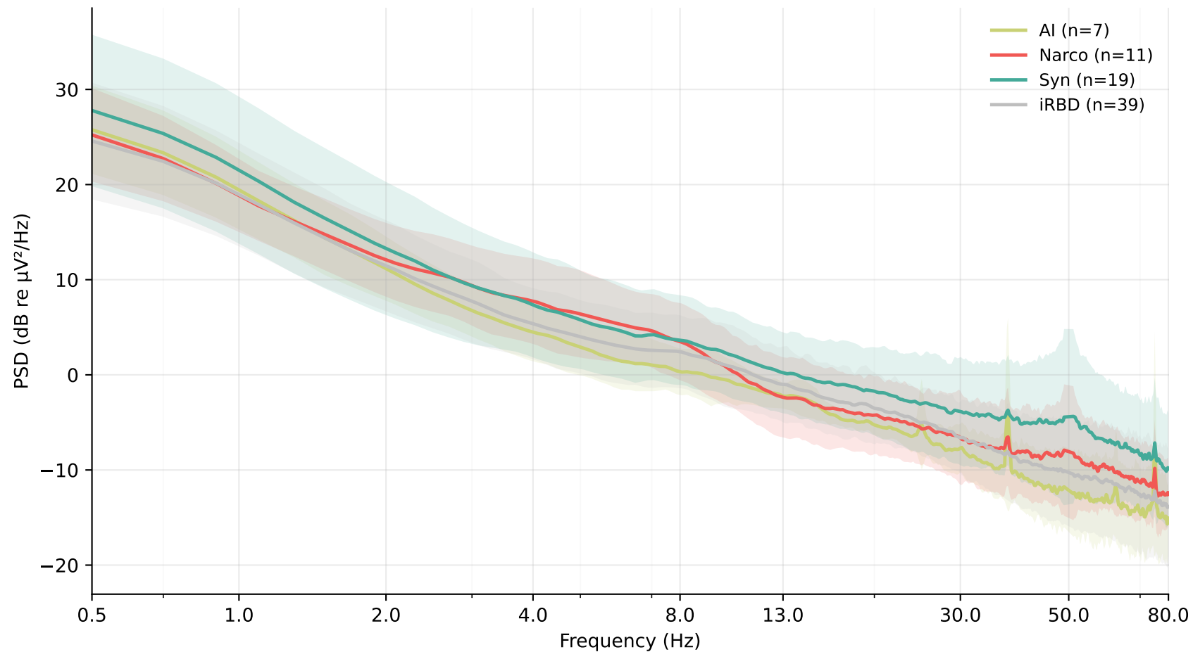
Mean PSD during REM sleep - Fp1-C3 (mean \pm std, Welch 4s/50%)
