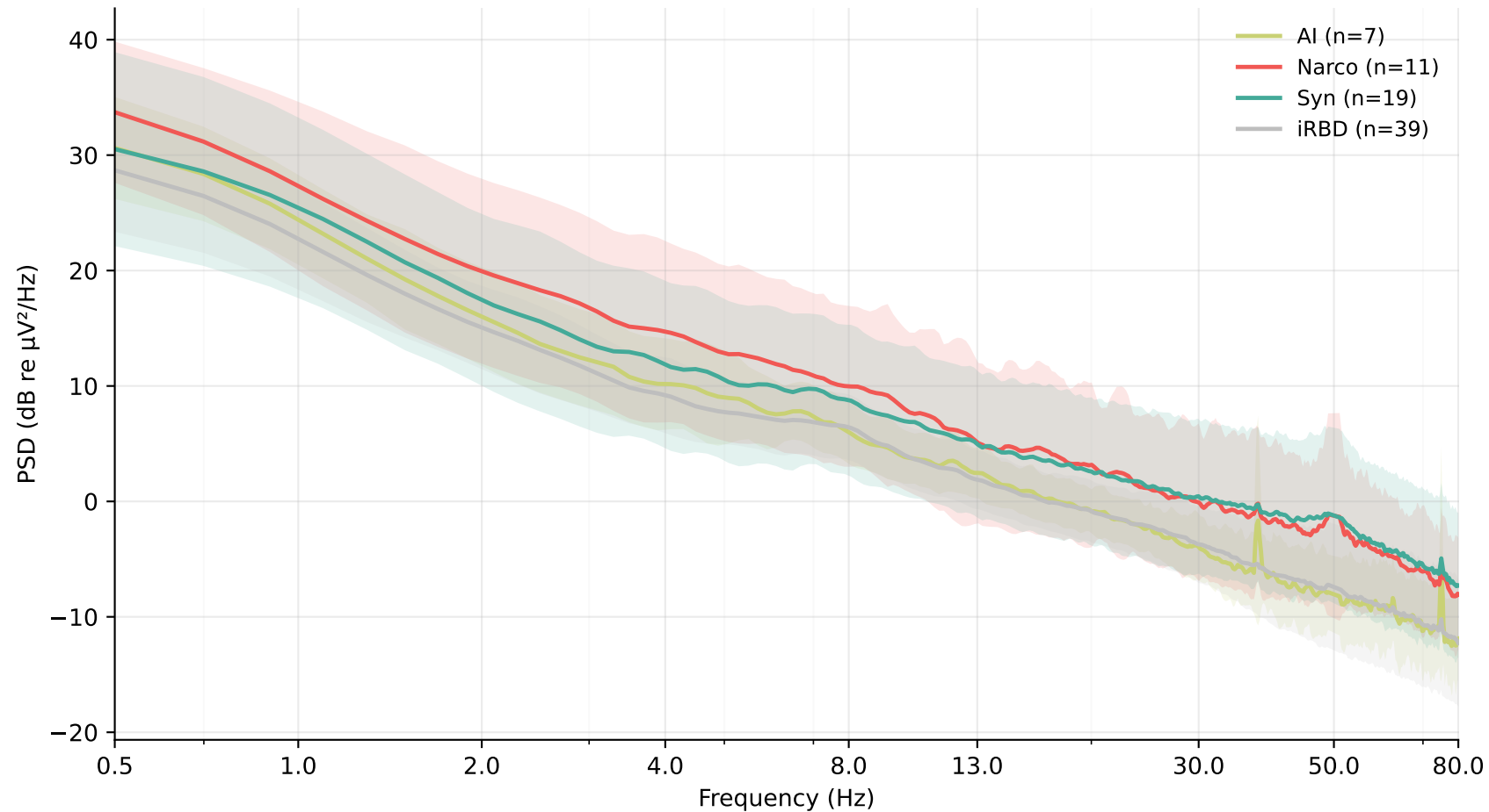
Mean PSD during REM sleep - Fp2-A1 (mean \pm std, Welch 4s/50%)
