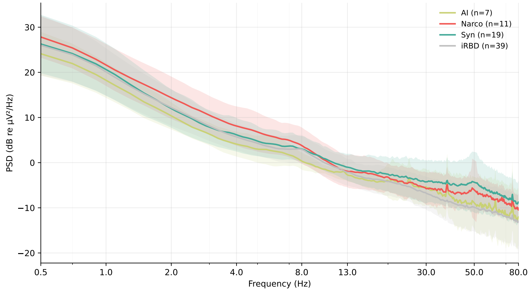
Mean PSD during REM sleep - Fp2-T4 (mean \pm std, Welch 4s/50%)
