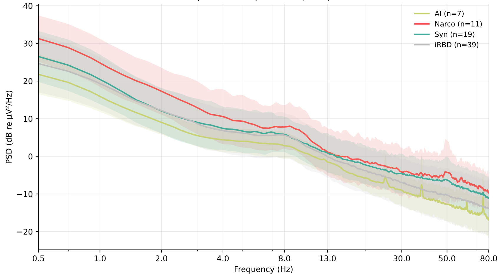
Mean PSD during REM sleep - T3-O1 (mean \pm std, Welch 4s/50%)
