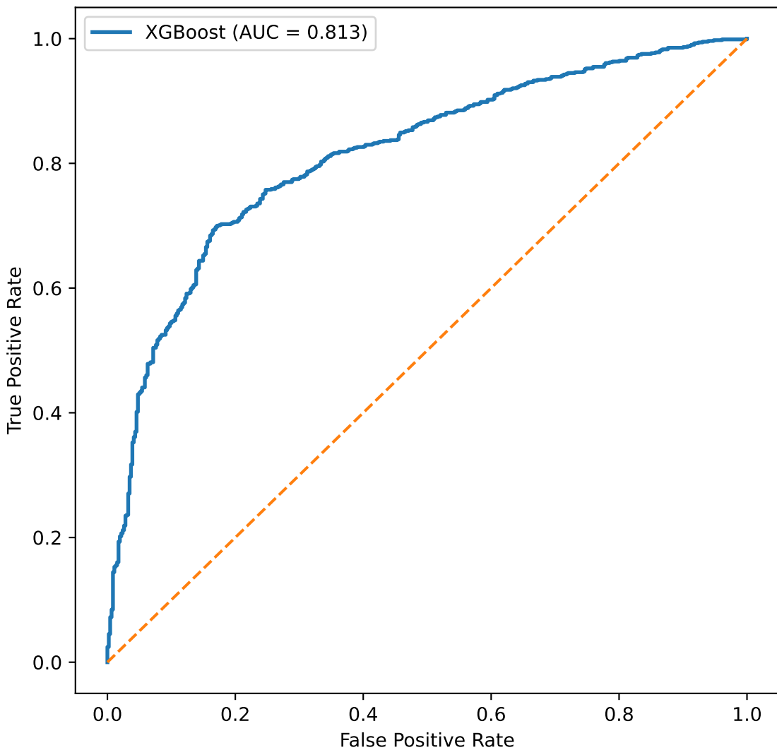
XGBoost ROC Curve
