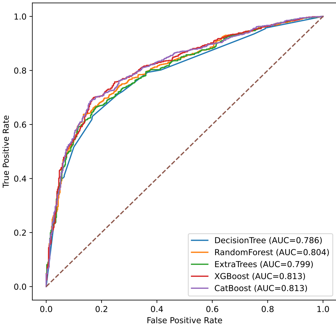
ROC Curves of Tree-Based Models
